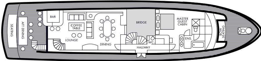
MIDDLE DECK
